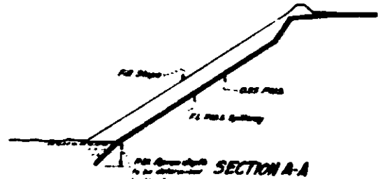
PLANT-MIXED SURFACING SPILLWAY DOWNDRAIN Scale: 1"=6'
