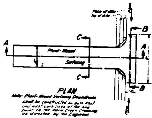
PLANT-MIXED SURFACING SPILLWAY DOWNDRAIN Scale: 1"=6'
